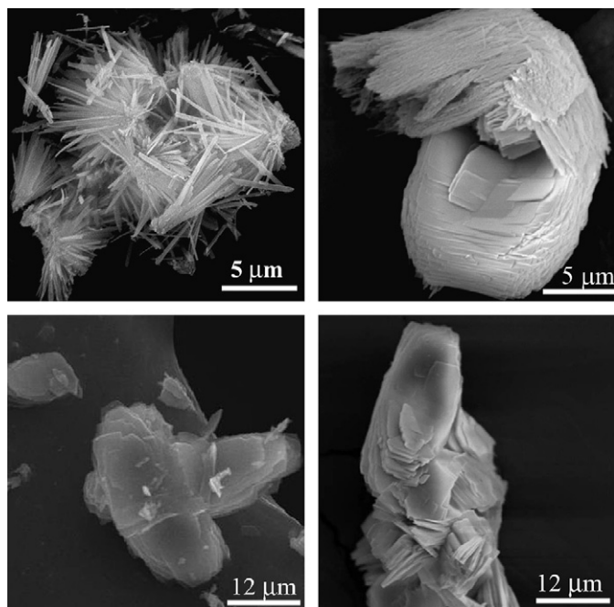
Fig. 3. SEM images of the samples FER-bmp-TMA obtained after 20 d of hydrothermal treatment (up, left), FER1 obtained after 14 d (up, right), FER-pyrr-TMA obtained at 10 d (down, left) and FER-pyrr obtained after 10 days (down, right).
