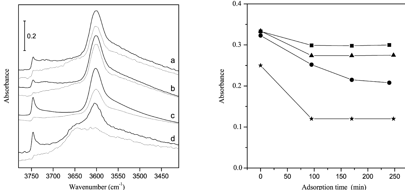
Fig. 4. Left: FTIR spectra in the \nu_{OH} region of ferrierite samples after outgassing at 400 °C (full lines) and subsequent adsorption of pyridine by contact with the amine vapour at 150 °C for 4 h (dotted lines): (a) FER-pyrr-TMA obtained after hydrothermal treatment for 7 d, (b) FER-pyrr at 10 d, (c) FER-bmp-TMA at 20 d and (d) FER1. Right: Intensity of the bridging OH band at 3601 \text{cm}^{-1} as a function of pyridine adsorption time, for samples FER-pyrr-TMA (triangles), FER-pyrr (squares), FER-bmp-TMA (circles) and FER1 (stars).
