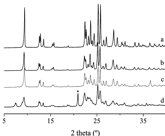
Fig. 2. XRD patterns of samples FER-pyrr (a), FER-pyrr-TMA (b) both obtained after 10 days of hydrothermal treatment, FER1 (c) obtained after 14 days and FER-bmp-TMA (d) obtained after 20 days. The peak highlighted with an asterisk corresponds to an unidentified dense phase. In all cases the pattern corresponds to the calcined sample.
