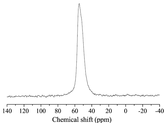
Fig. 5. ^{27}\text{Al} MAS NMR spectrum of the calcined FER-pyrr-TMA sample obtained after 10 days of heating.
