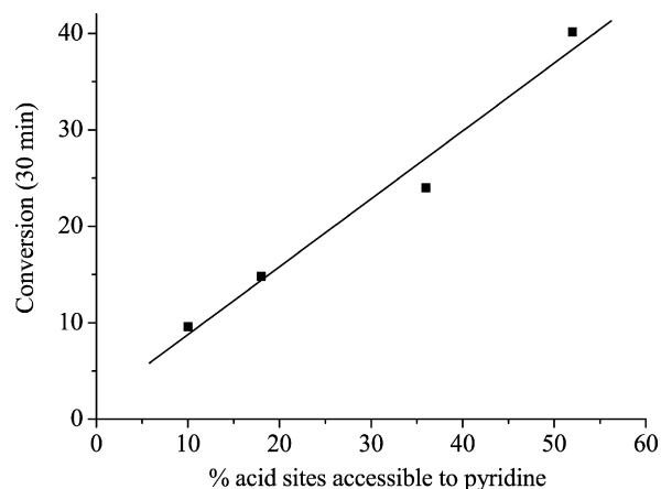
Fig. 7. Activity of the different samples in 1-butene isomerisation (time-on-stream = 30 min) as a function of the accessibility of pyridine to their acid sites in the IR experiments.
