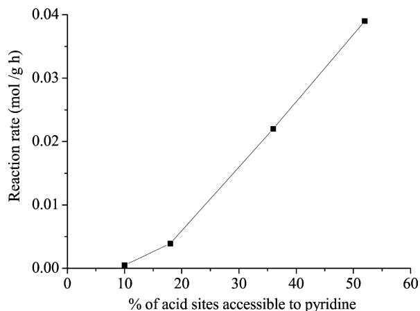
Fig. 6. Activity of the different samples in m -xylene isomerisation as a function of the accessibility of pyridine to their acid sites in the IR experiments.
